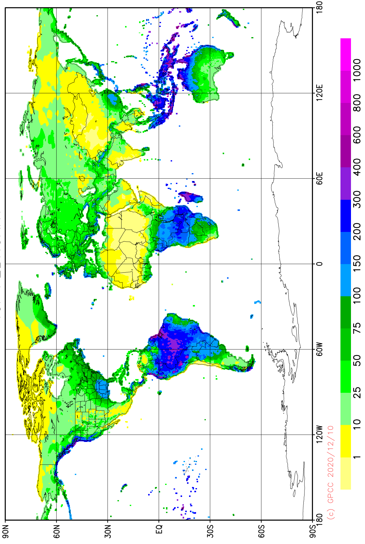
GPCC Precipitation Normals in mm/month (Version 2020) per 0.25 degree grid for FEBRUARY
