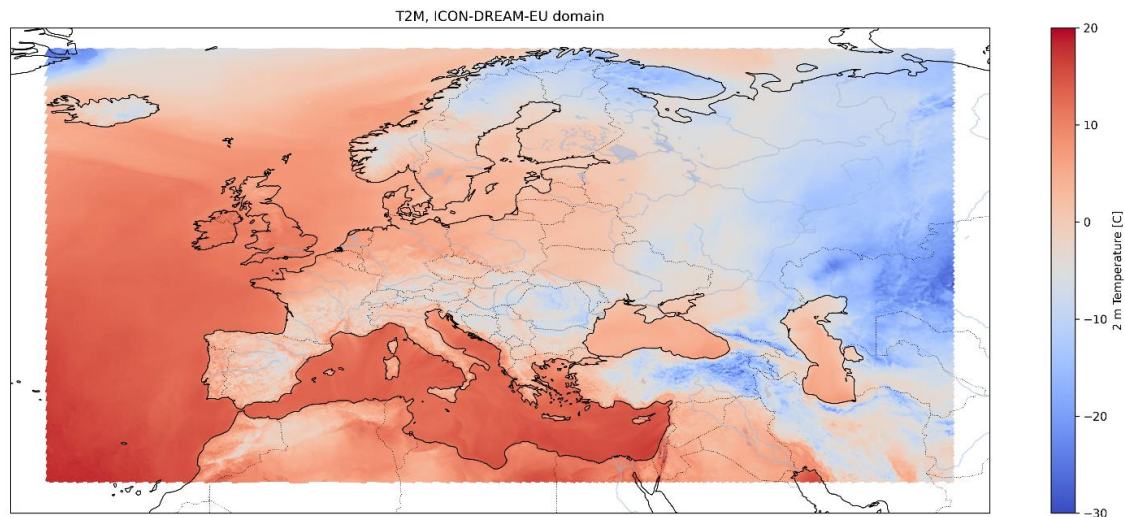
Figure 1: ICON-DREAM-EU domain illustrated with the 2m temperature.
